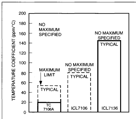
Figure 10. Analog Common Temperature Coefficient
