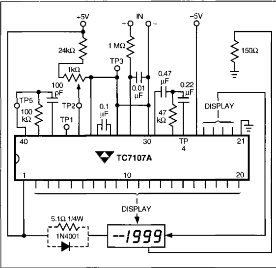
Figure 15. Diode or Resistor Limits Package Power Dissipation
