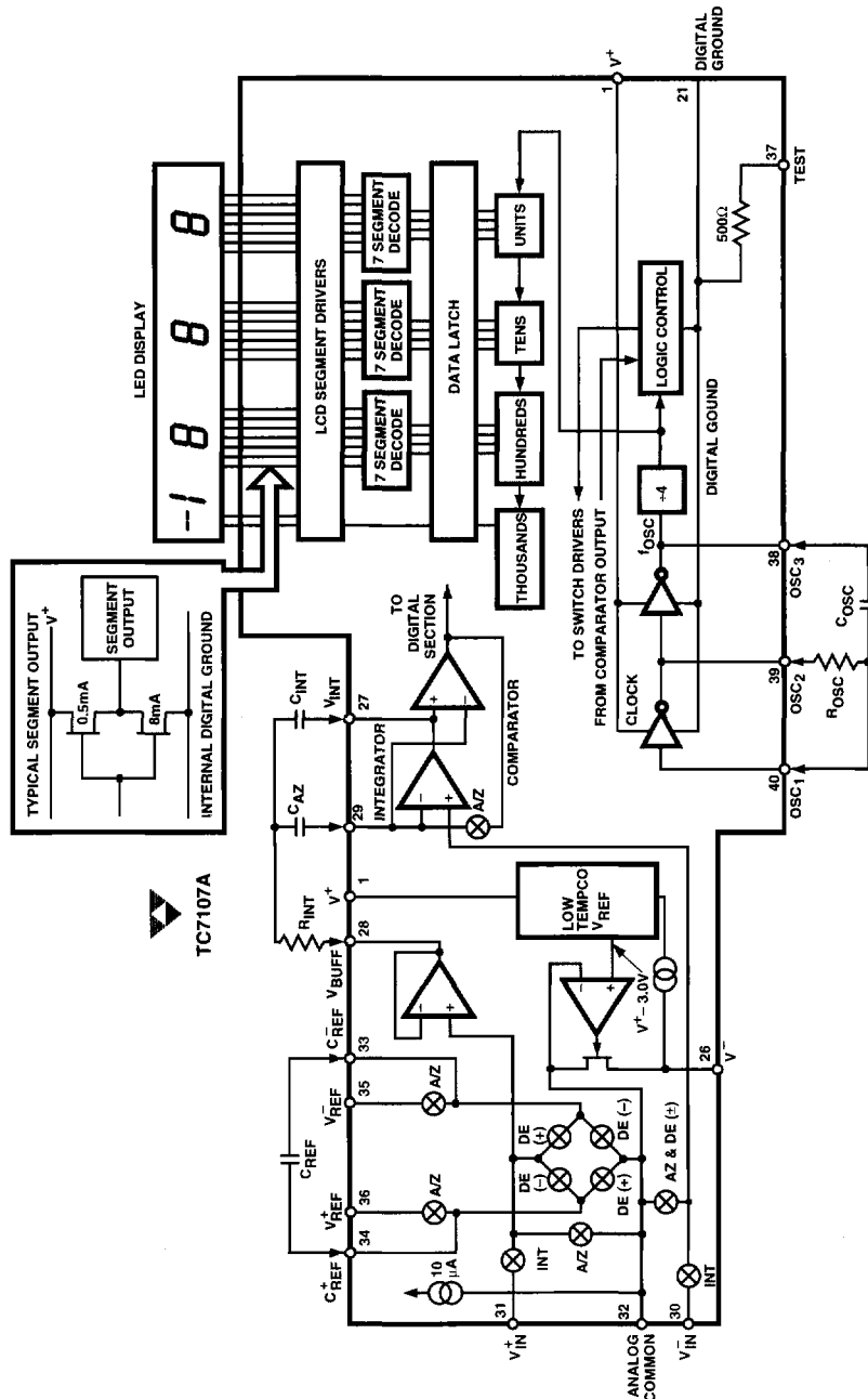
Figure 5. TC7107A Block Diagram
