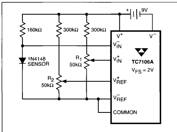
Figure 19. Temperature Sensor
