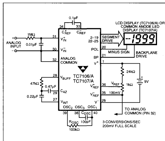
Figure 1. TC7106/A/7/A Typical Operating Circuit
