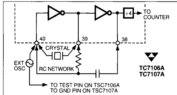
Figure 6. Clock Circuits
