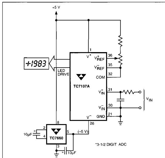
Figure 13. Negative Power Supply Generation with TC7660
