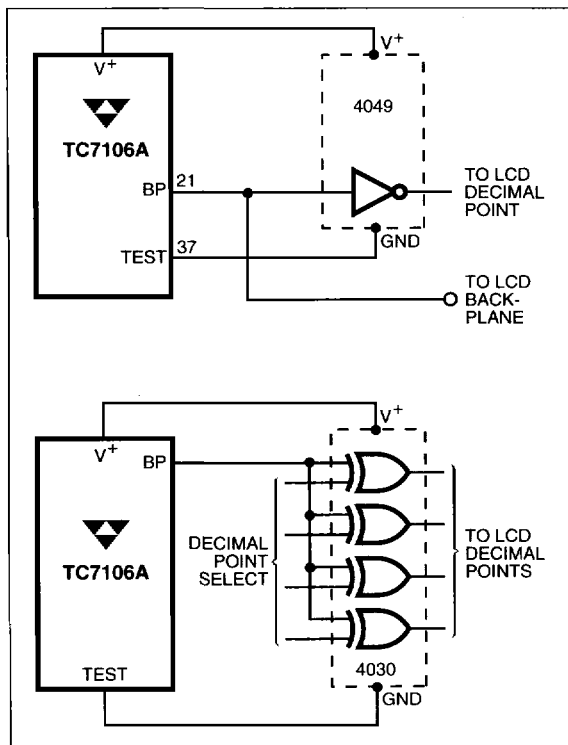
Figure 16. Decimal Point Drive Using TEST as Logic Ground
