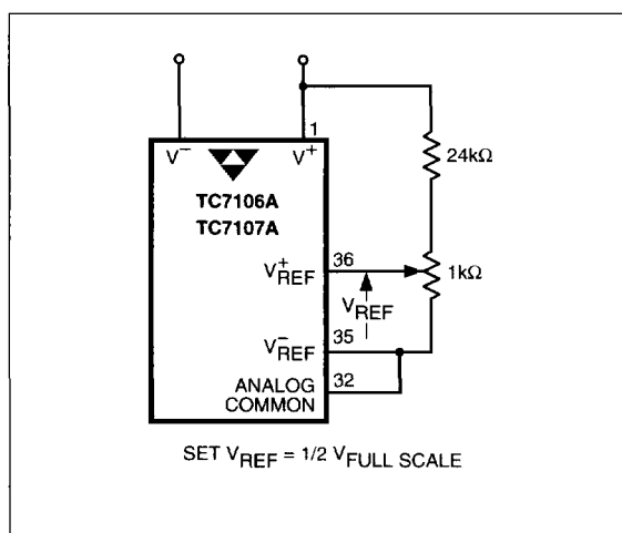
Figure 11. Internal Voltage Reference Connection
