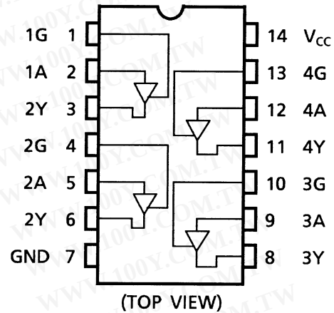
TC74HC126A
