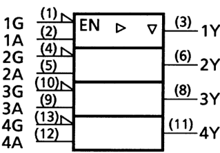
TC74HC126A
