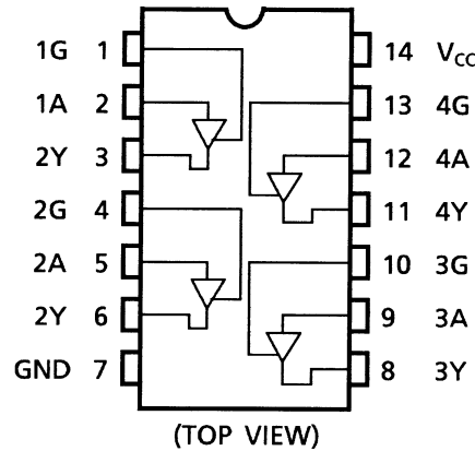
TC74HC126A
