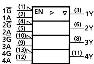
TC74HC125A
