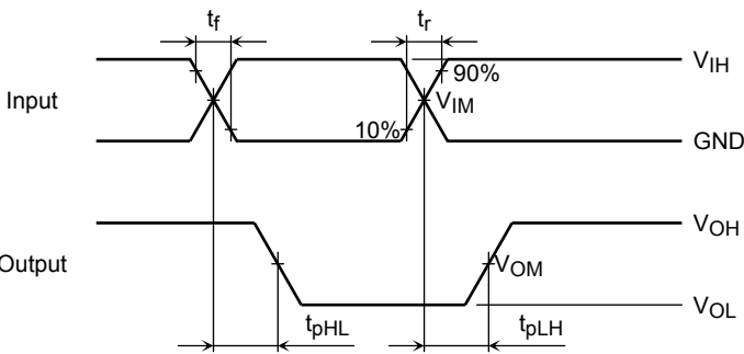
Figure 2 t_{pLH} , t_{pHL}
