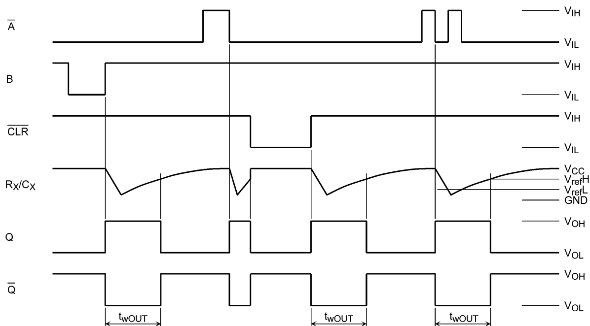
Fig. 11.2 TC74VHC221AF, TC74VHC221AFK
