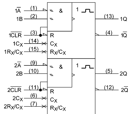
TC74VHC221AF,TC74VHC221AFK
