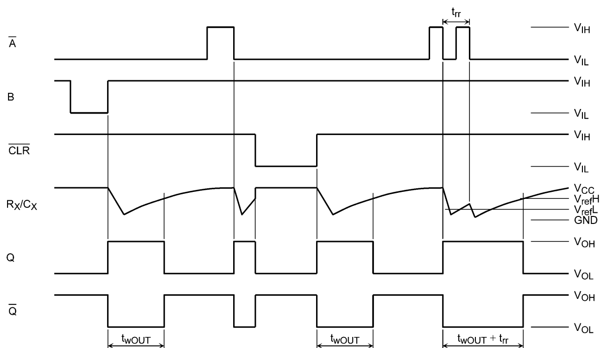
Fig. 11.1 TC74VHC123AF, TC74VHC123AFK
