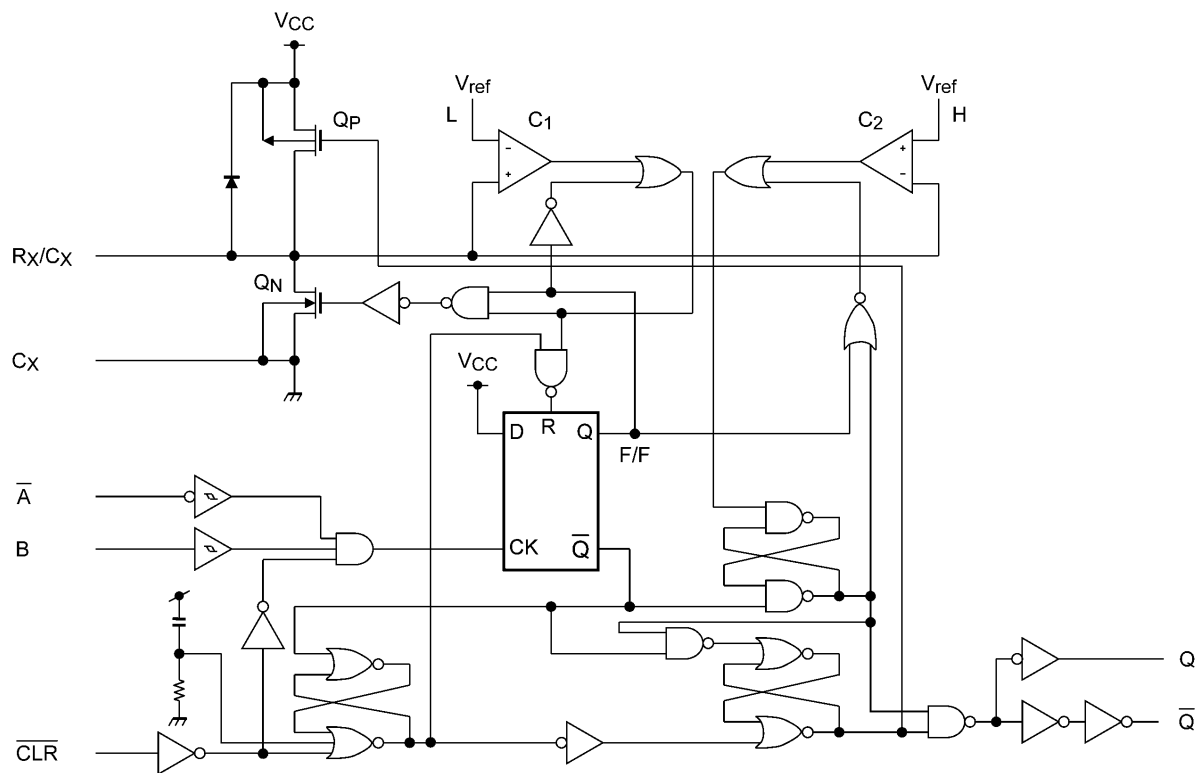
Fig. 10.1 TC74VHC123AF, TC74VHC123AFK
