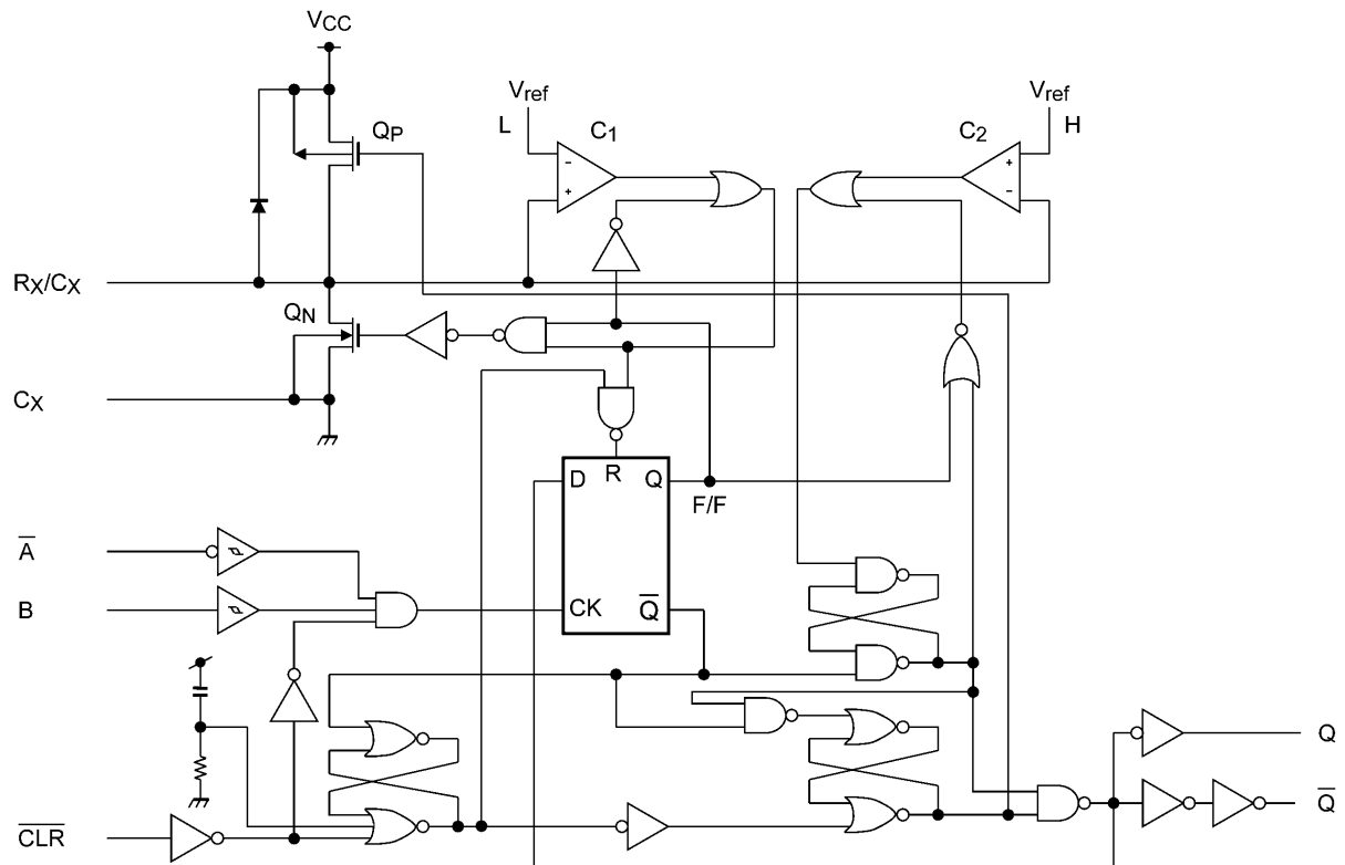
Fig. 10.2 TC74VHC221AF, TC74VHC221AFK
