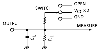
Figure 1 AC Characteristics Measurement Circuit
