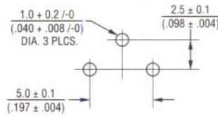
Suggested PCB Layout – Styles K, P, W
