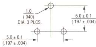
Suggested PCB Layout – Style F
