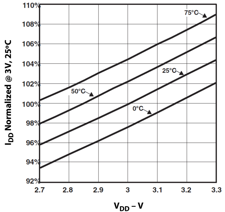
Figure 15: Normalized I_{DD} vs. V_{DD} and Temperature
