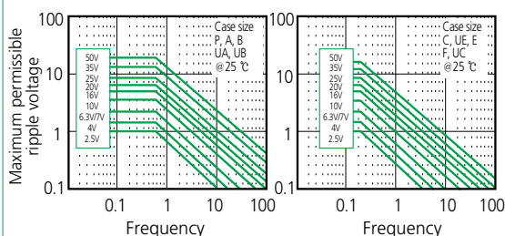
Fig. 7 Maximum permissible ripple voltage(C, D)
