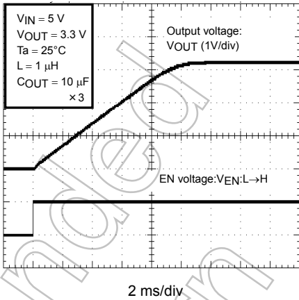
Startup Characteristics ( C_{SS} = 0.1\text{ }\mu\text{F} )
