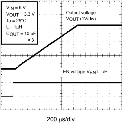
Startup Characteristics (Internal Soft-Start Time)
