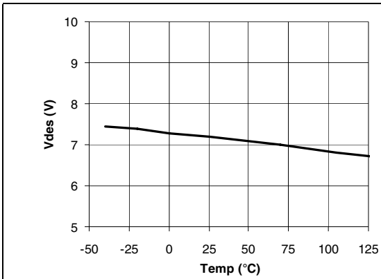
Figure 12. High level output voltage vs temp.
