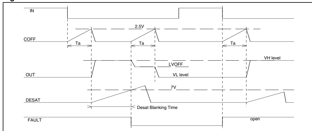
Figure 7. Desaturation fault
