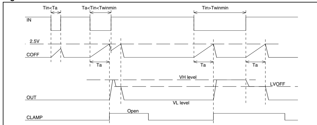
Figure 7. Desaturation fault
