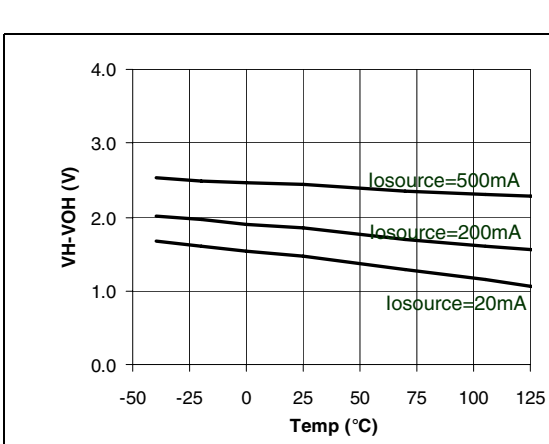
Figure 12. High level output voltage vs temp.
