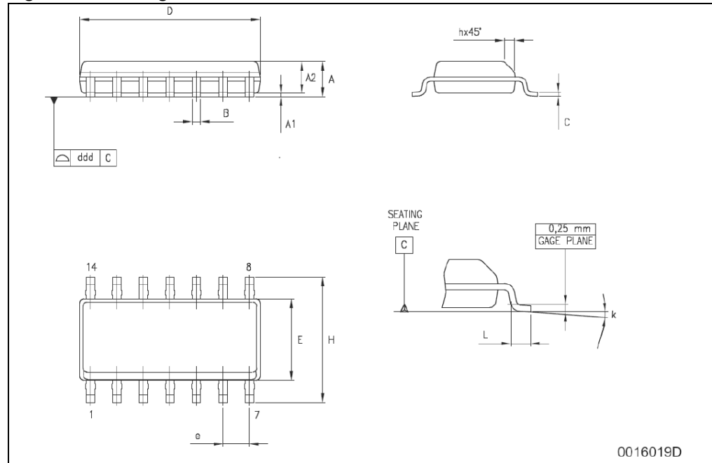
Figure 17. Package dimensions
