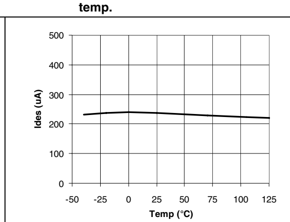
Figure 13. Desaturation source current vs temp.
