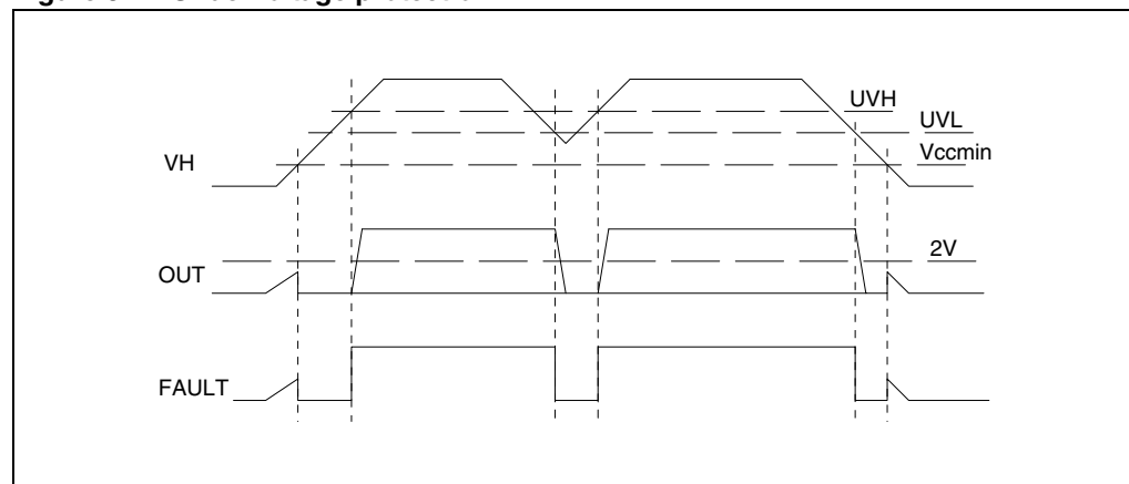
Figure 3. Undervoltage protection
