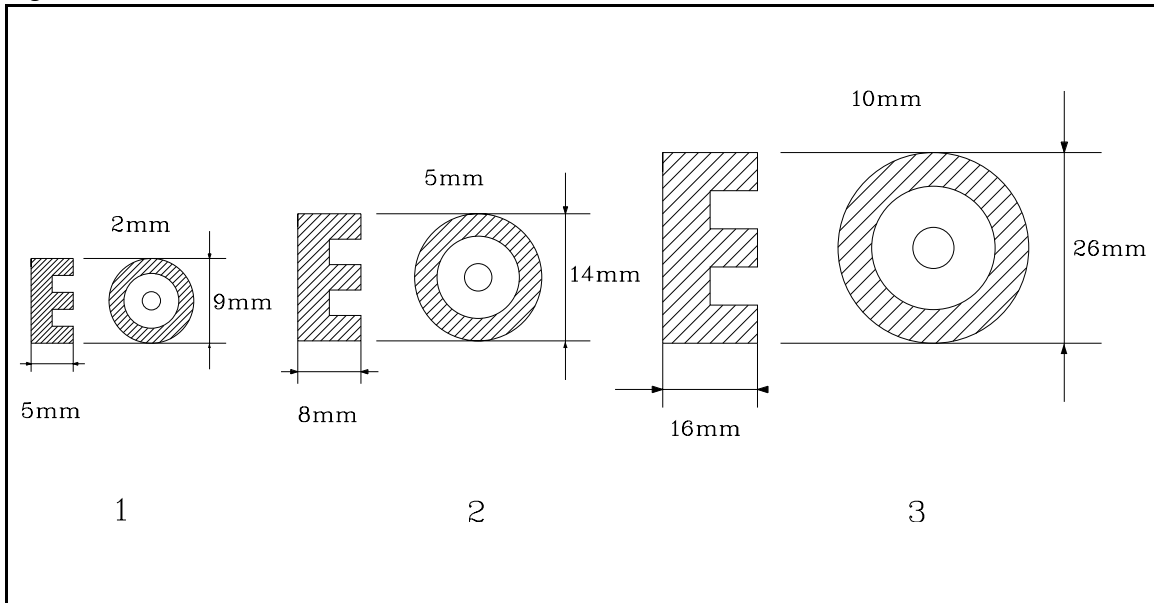
Figure 4. Detection distance
