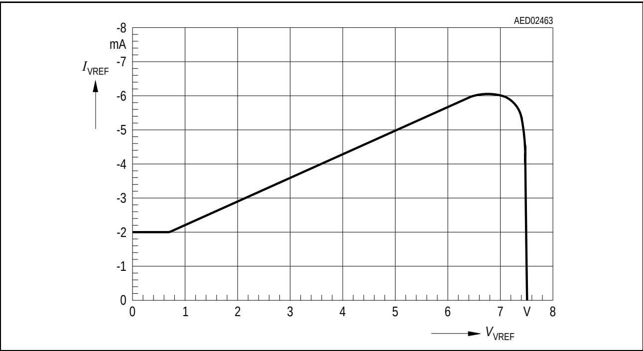
Figure 4 Foldback Characteristic of Pin 2 ( V_{REF} )
