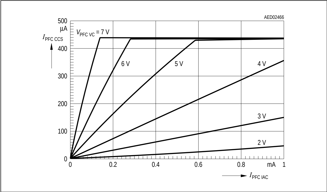
Figure 7 Multiplier Linearity
