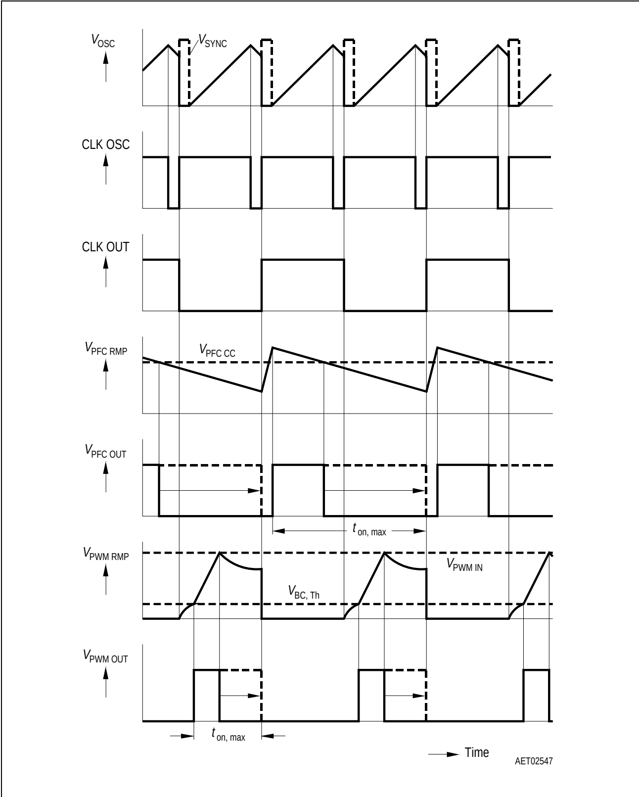
Figure 19 Timing Diagram with Synchronization ( f_{\text{SYNC}} > f_{\text{OSC}} )
