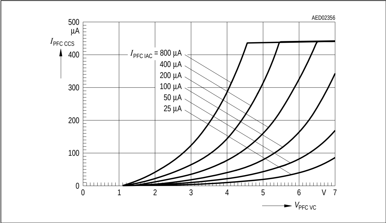
Figure 8 Multiplier Dynamic
