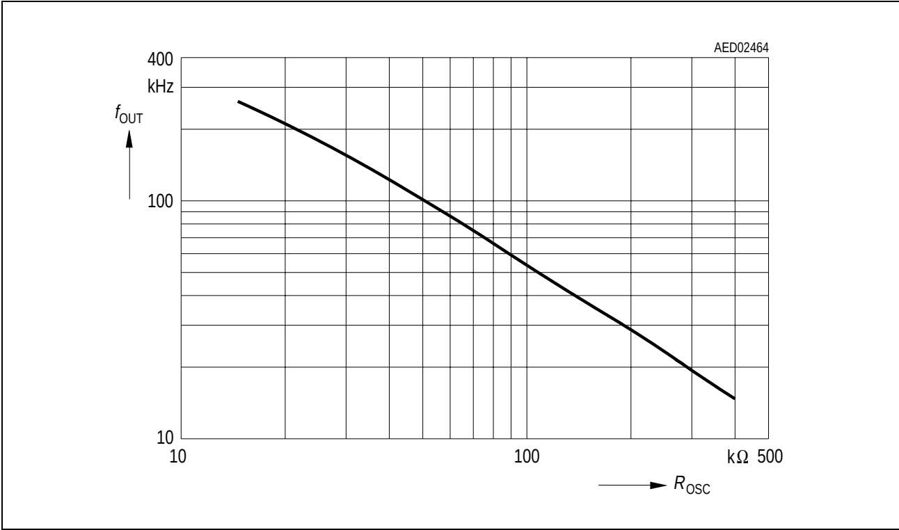
Figure 5 PFC/PWM Frequency
