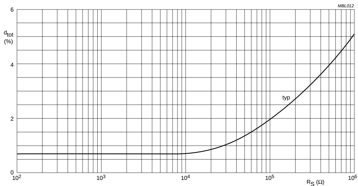
Fig.8 Total harmonic distortion as a function of R_S in the circuit of Fig. 3; P_o = 3,5 \text{ W} ; f = 1 \text{ kHz} .
