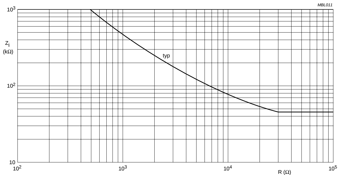
Fig.7 Input impedance as a function of R in circuit of Fig. 3; C = 1 \mu\text{F} ; f = 1 \text{ kHz} .
