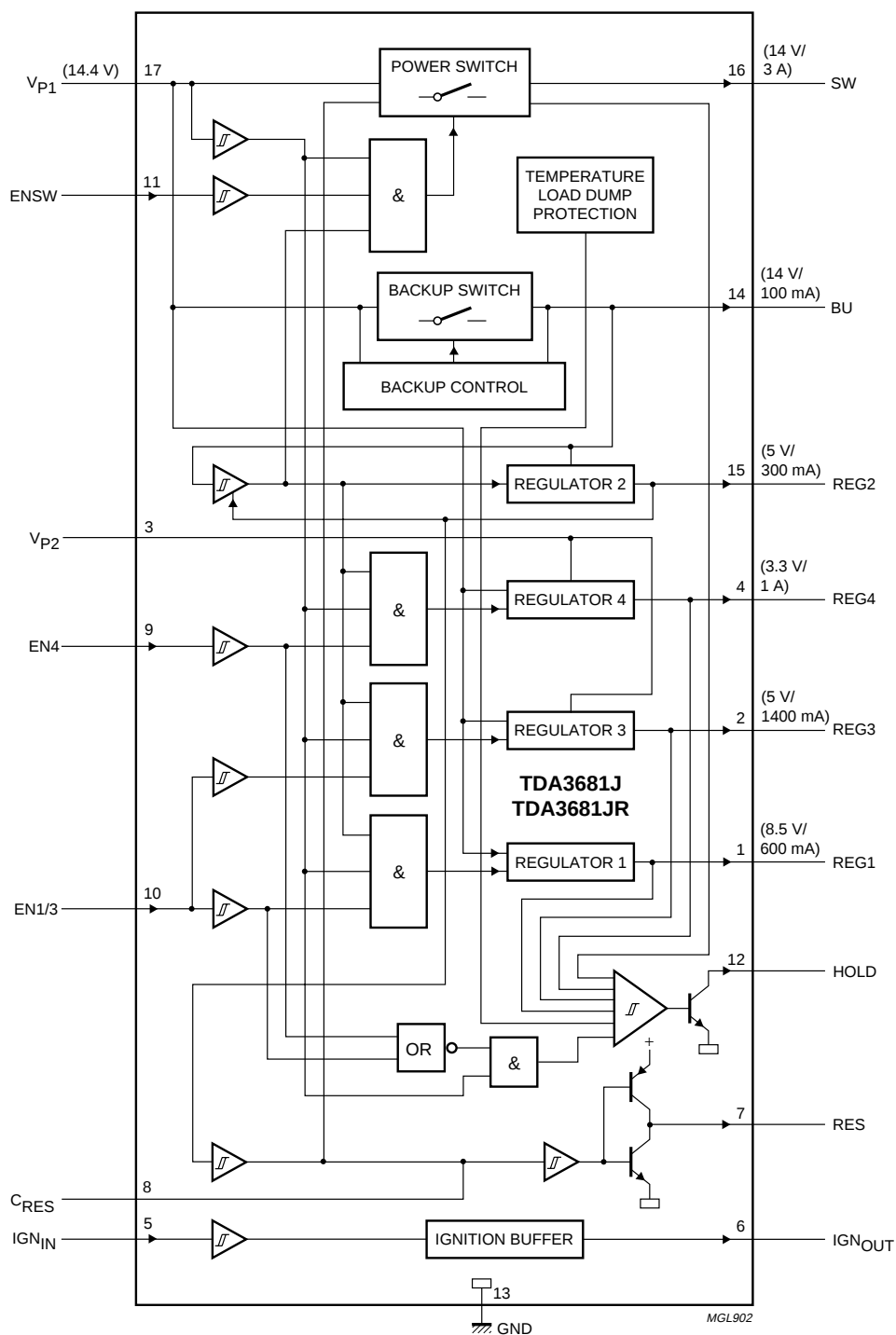
Fig.1 Block diagram of TDA3681J and TDA3681JR.
