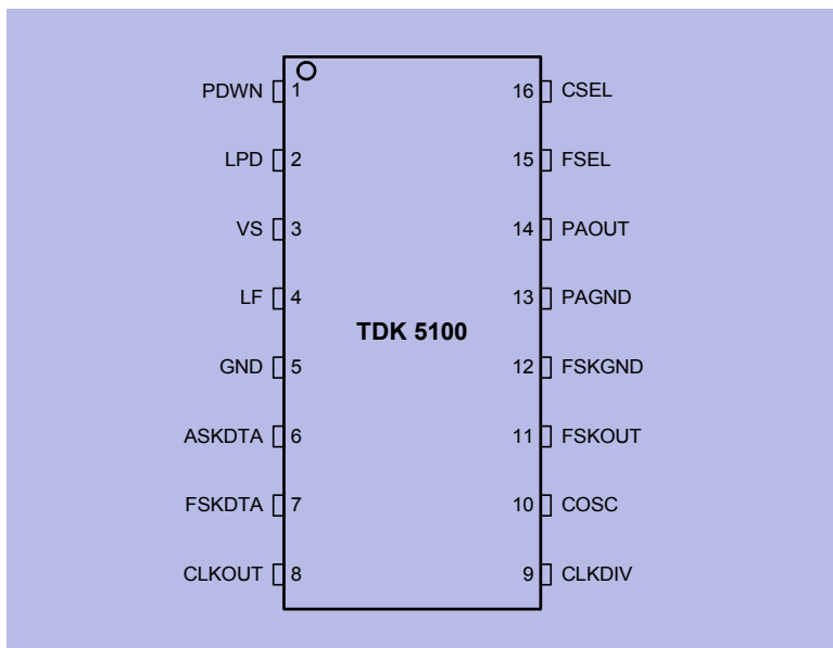
Figure 2-1 IC Pin Configuration
