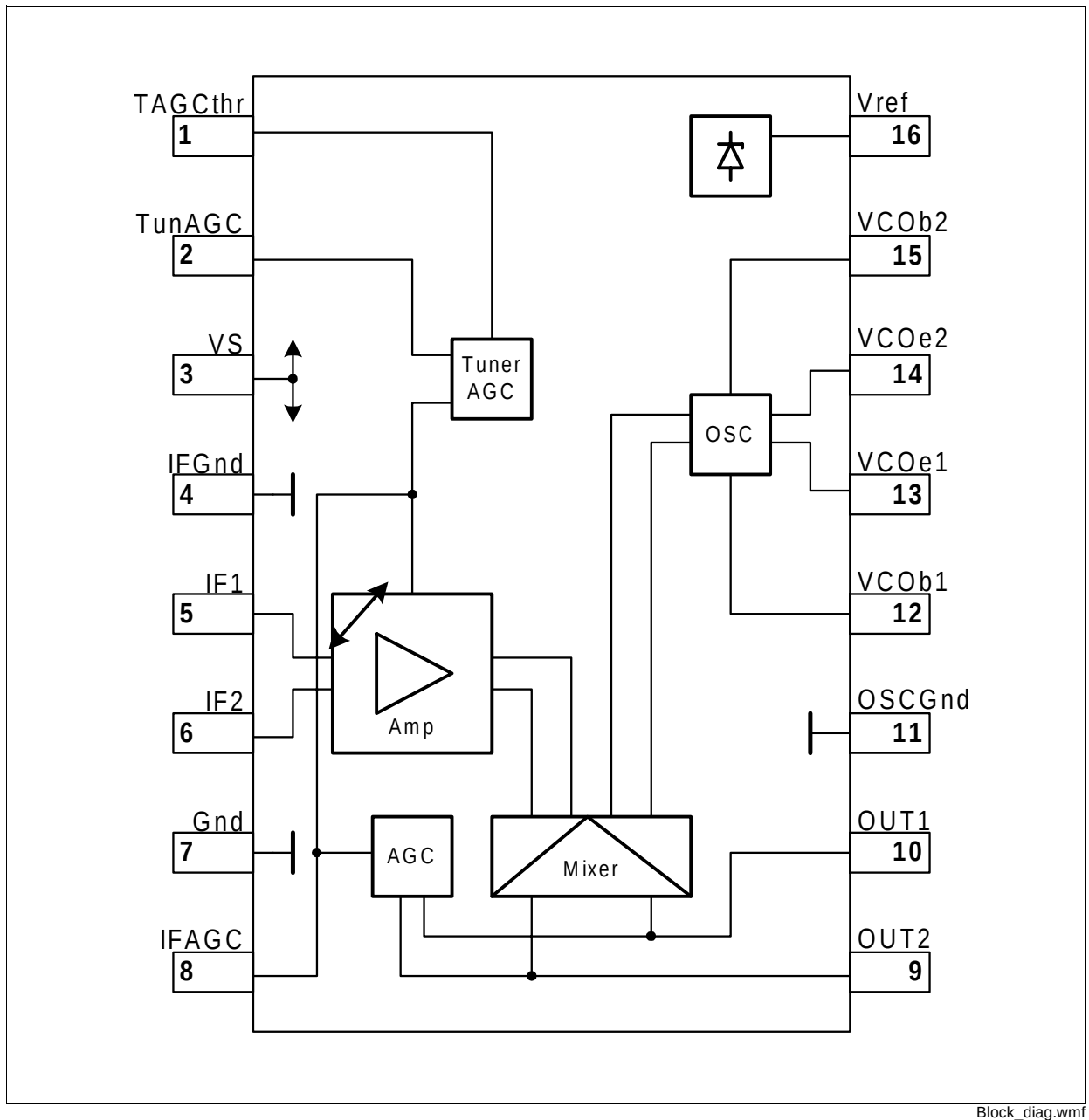
Figure 2-3 Block Diagram
