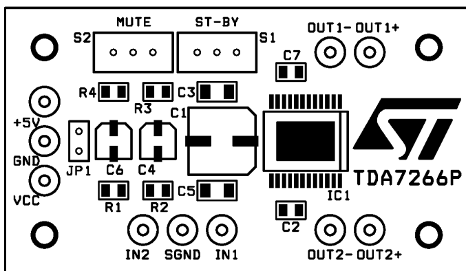
Figure 8. PCB Component Layout
