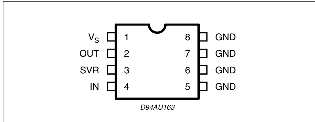
Figure 2. Pin connection (top view, PCB view)
