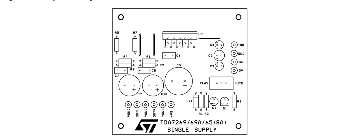
Figure 9. Component Layout
