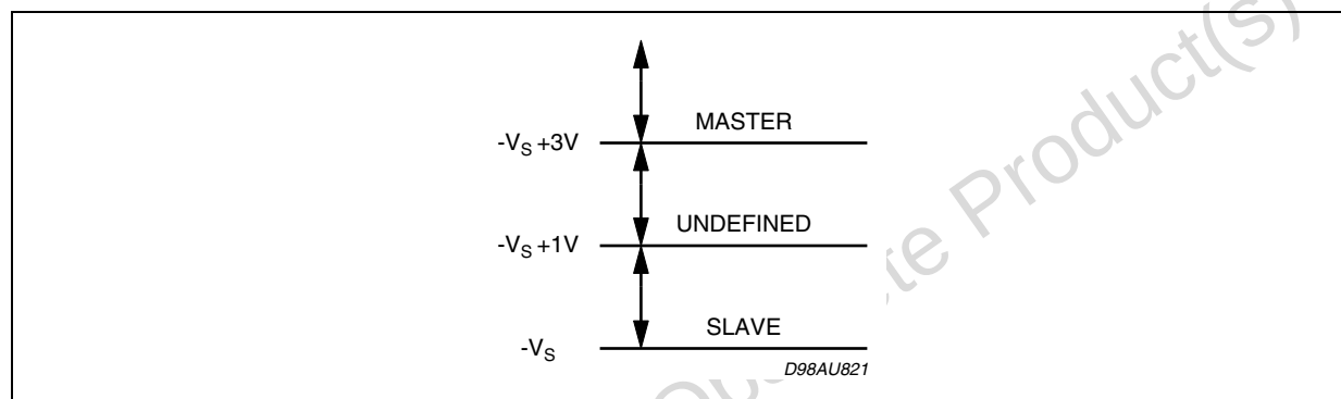
Figure 5. Slave function: pin 4 (Ref to pin 8 -Vs)
