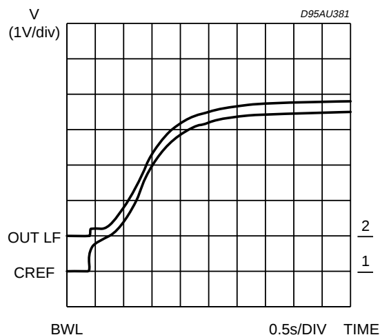
Figure 9: Power on Time Constant vs Cref Capacitor C_{REF} = 10\mu F
