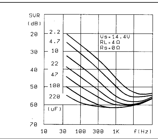
Figure 10. Supply volt. rejection vs. frequency for a different values of C6 capacitor
