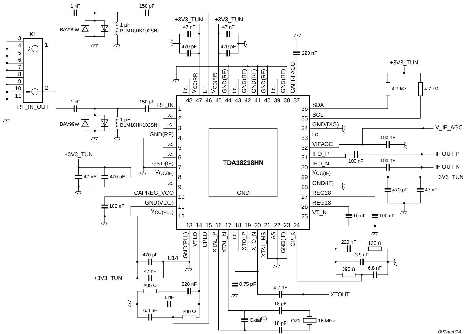
Fig 3. Application diagram
