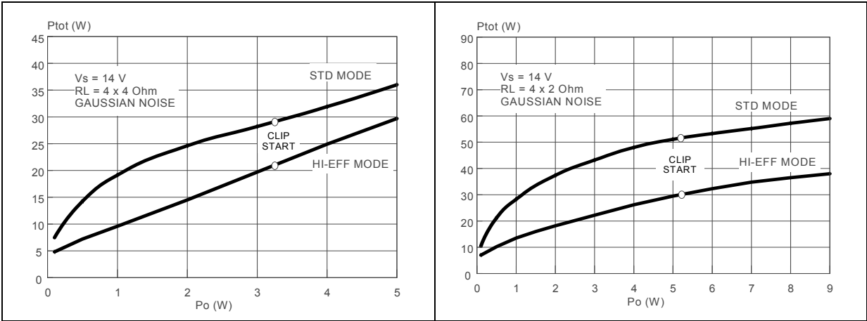
Figure 17. Power dissipation vs. average output power (audio program simulation, 4 \Omega ) Figure 18. Power dissipation vs. average output power (audio program simulation, 2 \Omega )
