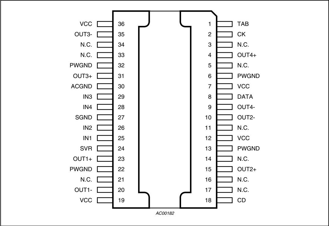
Figure 4. PowerSO36 (slug-up) pins connection diagram (top of view)
