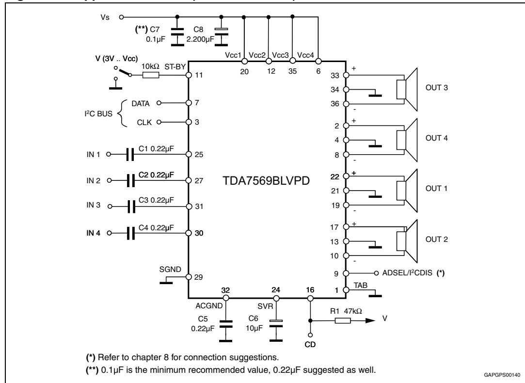
Figure 3. Application circuit (TDA7569BLVPD)
