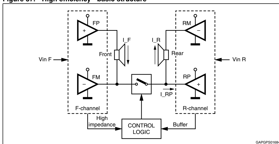
Figure 37. High efficiency - basic structure
