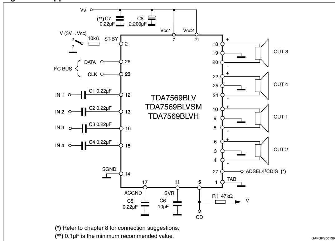
Figure 2. Application circuit
