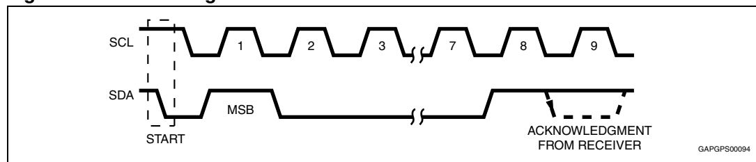
Figure 40. Acknowledge on the I 2 C bus
