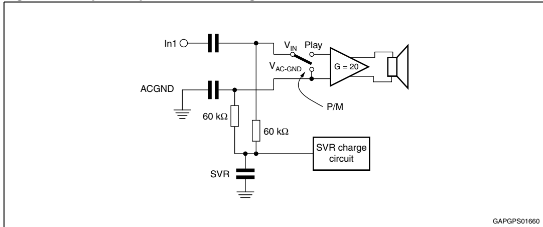
Figure 36. Inputs impedance matching circuit
