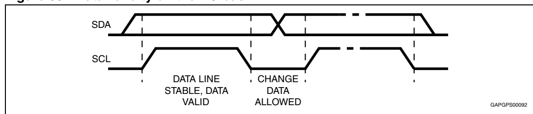
Figure 39. Timing diagram on the I 2 C bus
