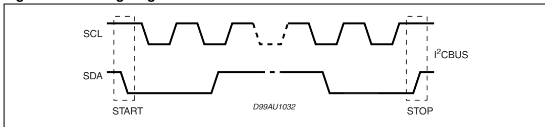
Figure 27. Timing diagram on the I 2 C bus
