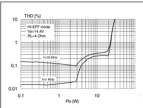
Figure 7. Distortion vs. output power
