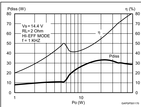
Figure 20. Power dissipation vs. average Po (2 \Omega , HI-EFF mode)
