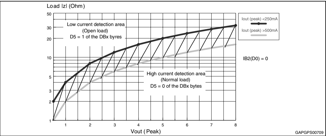
Figure 30. Current detection high: load impedance |Z| vs. output peak voltage
