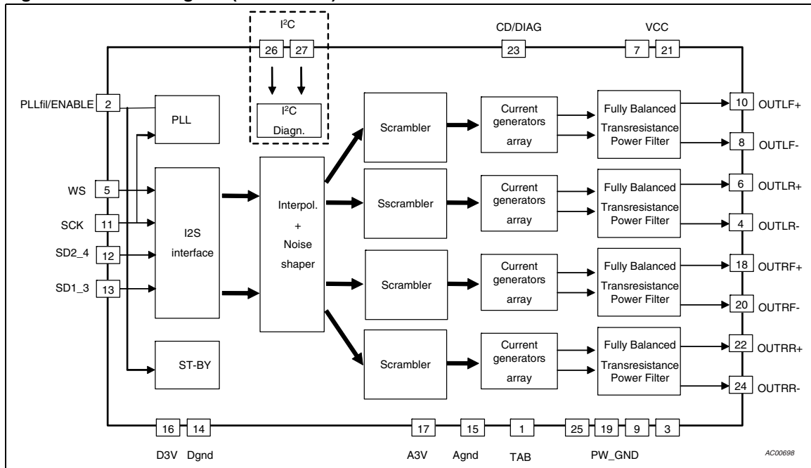
Figure 1. Block diagram (Flexiwatt27)
