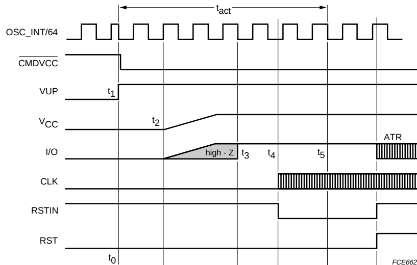
Fig.5 Activation sequence.
