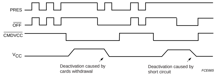
Fig. 7 Behaviour of \overline{\text{OFF}} , \overline{\text{CMDVCC}} , \text{PRES} and \text{V}_{\text{CC}} (see also application note AN97036 for software decision algorithm on \overline{\text{OFF}} signal).
