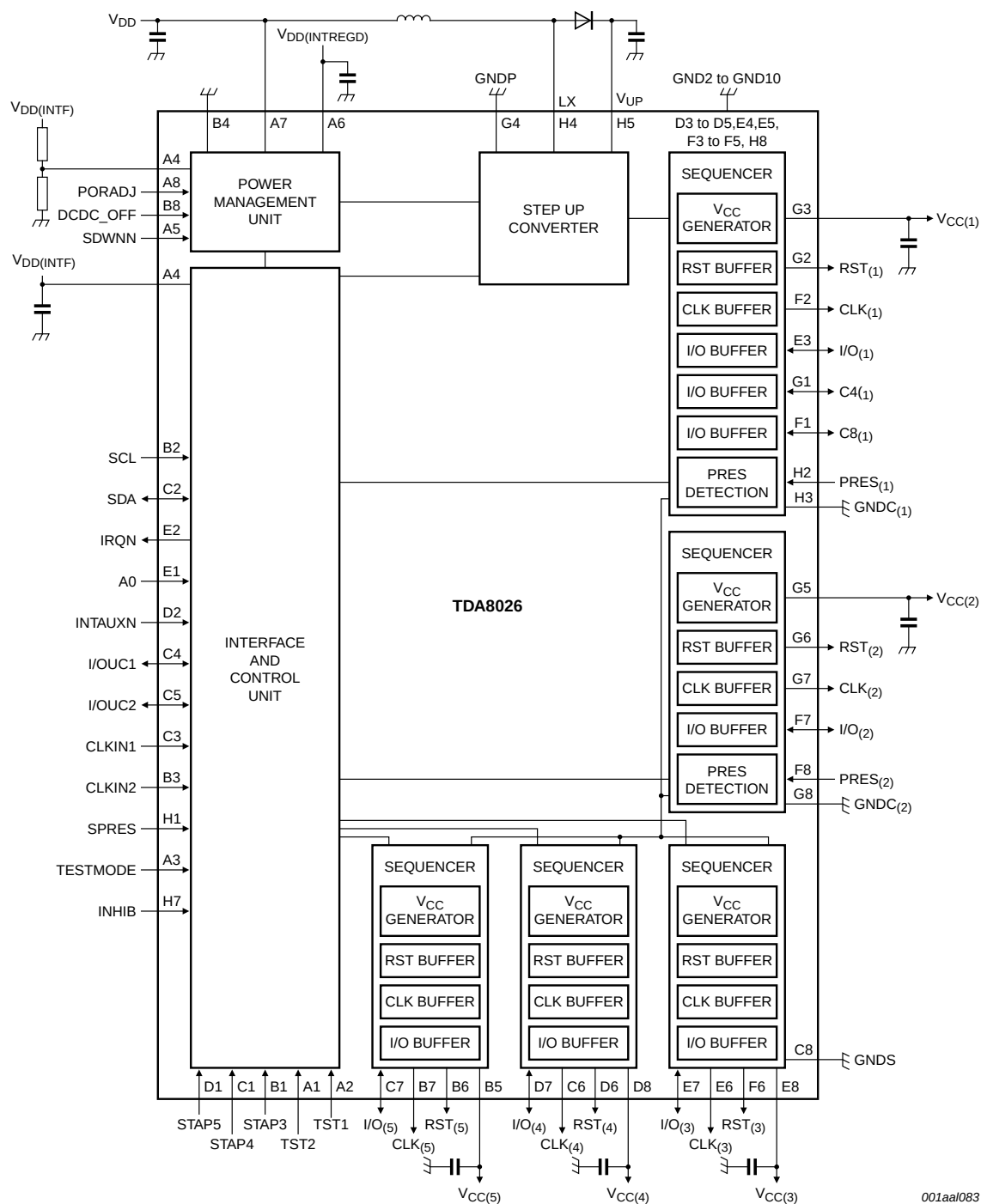
Fig 1. TDA8026 Block diagram
