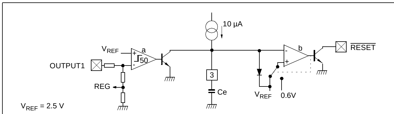
Figure 3: Reset Diagram
