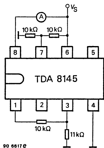
Figure 5. Test circuit 3
