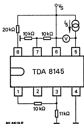
Figure 7. Test circuit 5
