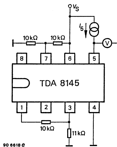
Figure 6. Test circuit 4
