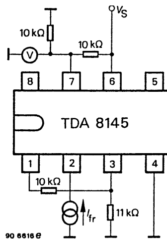
Figure 4. Test circuit 2
