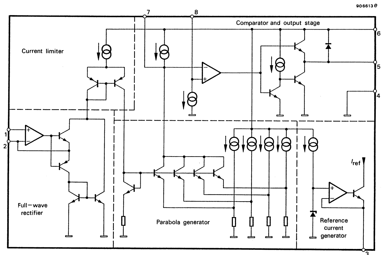
Figure 1. Block diagram
