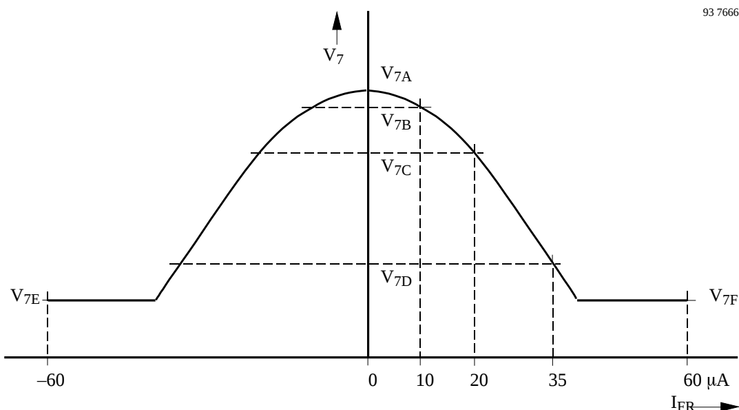
Figure 2. Parabola coefficients
