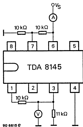
Figure 3. Test circuit 1
