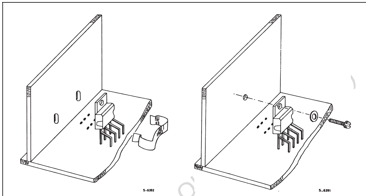
Figure 6. Mounting examples
