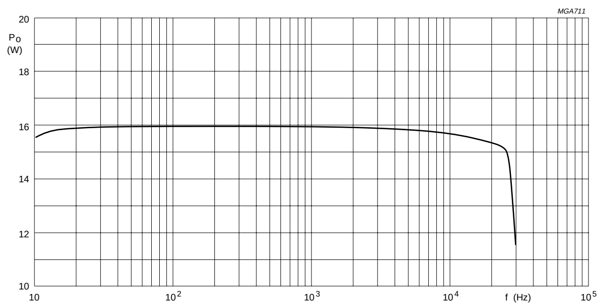
Fig.14 Power bandwidth as a function of frequency; THD = 0.5%, V_p = 14.4 \text{ V} , R_L = 4 \Omega .
