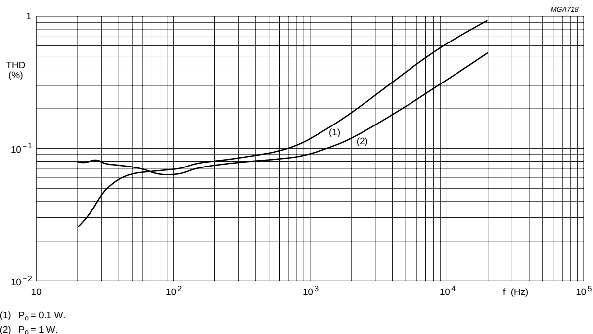
Fig.21 Total harmonic distortion as a function of frequency; V_P = 14.4 \text{ V} , R_L = 2 \Omega .
