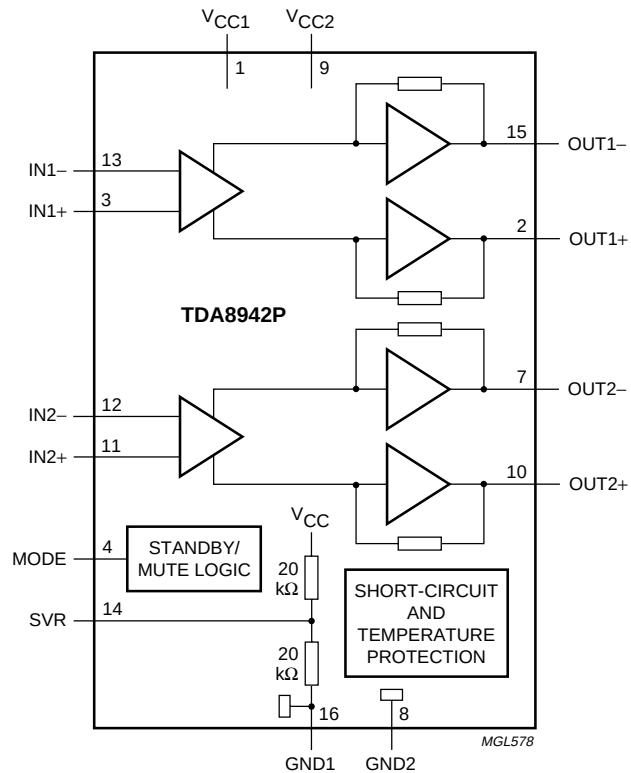
Fig 1. Block diagram.
