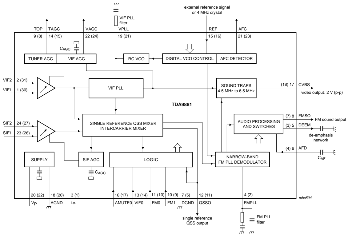
Fig 1. Block diagram.
