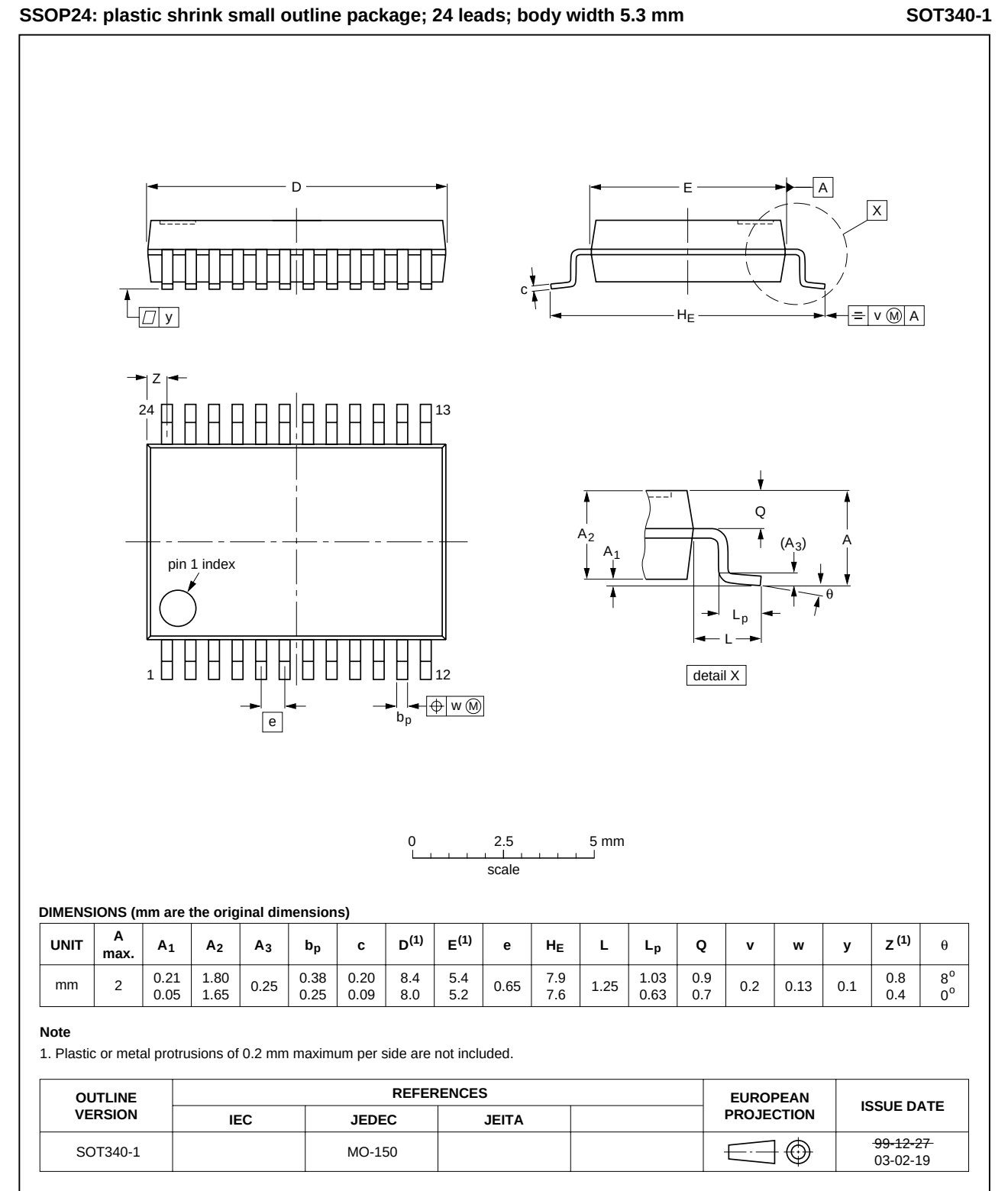
Fig 28. Package outline SOT340-1 (SSOP24)
