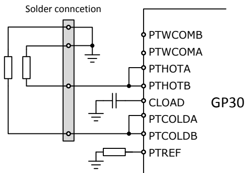
Figure 3-7 2-wire temperature sensors
