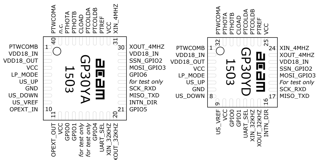
Figure 2-5 GP30 Pinout
