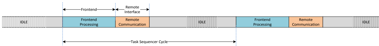
Figure 7-2 Time Conversion Mode
