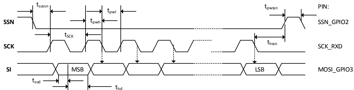
Figure 2-2 SPI Write
