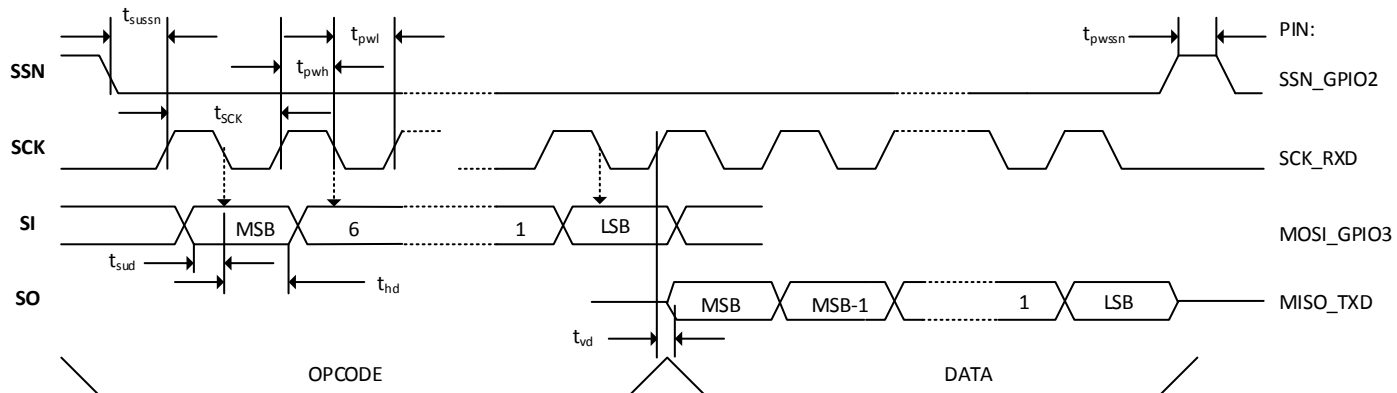
Figure 2-3 SPI Read
