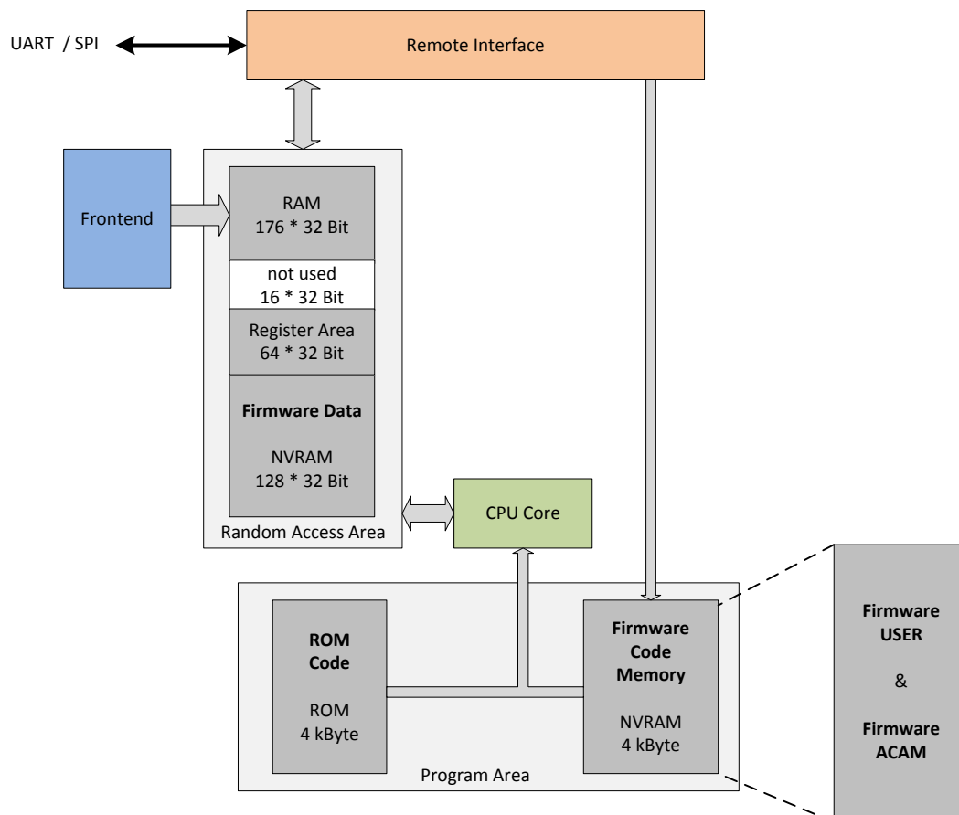
Figure 7-1 Memory organization
