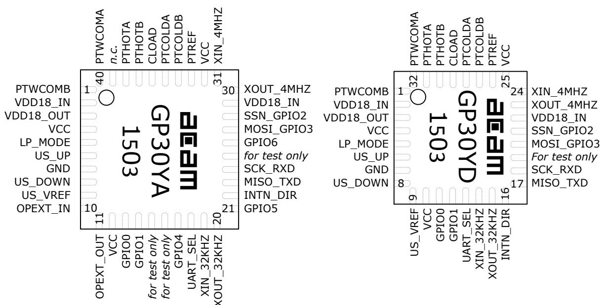
Figure 2-5 GP30 Pinout
