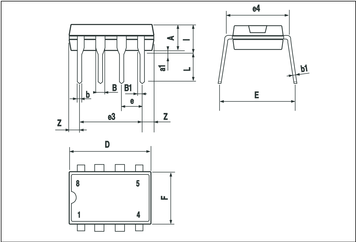
Figure 11. Package dimensions
