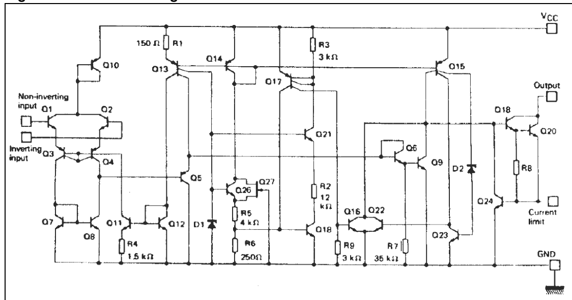
Figure 2. Schematic diagram
