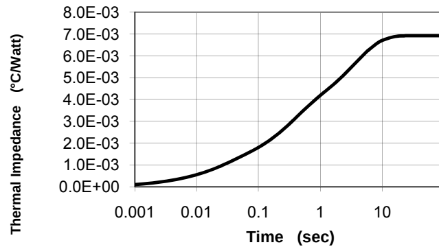
MAXIMUM TRANSIENT THERMAL IMPEDANCE
