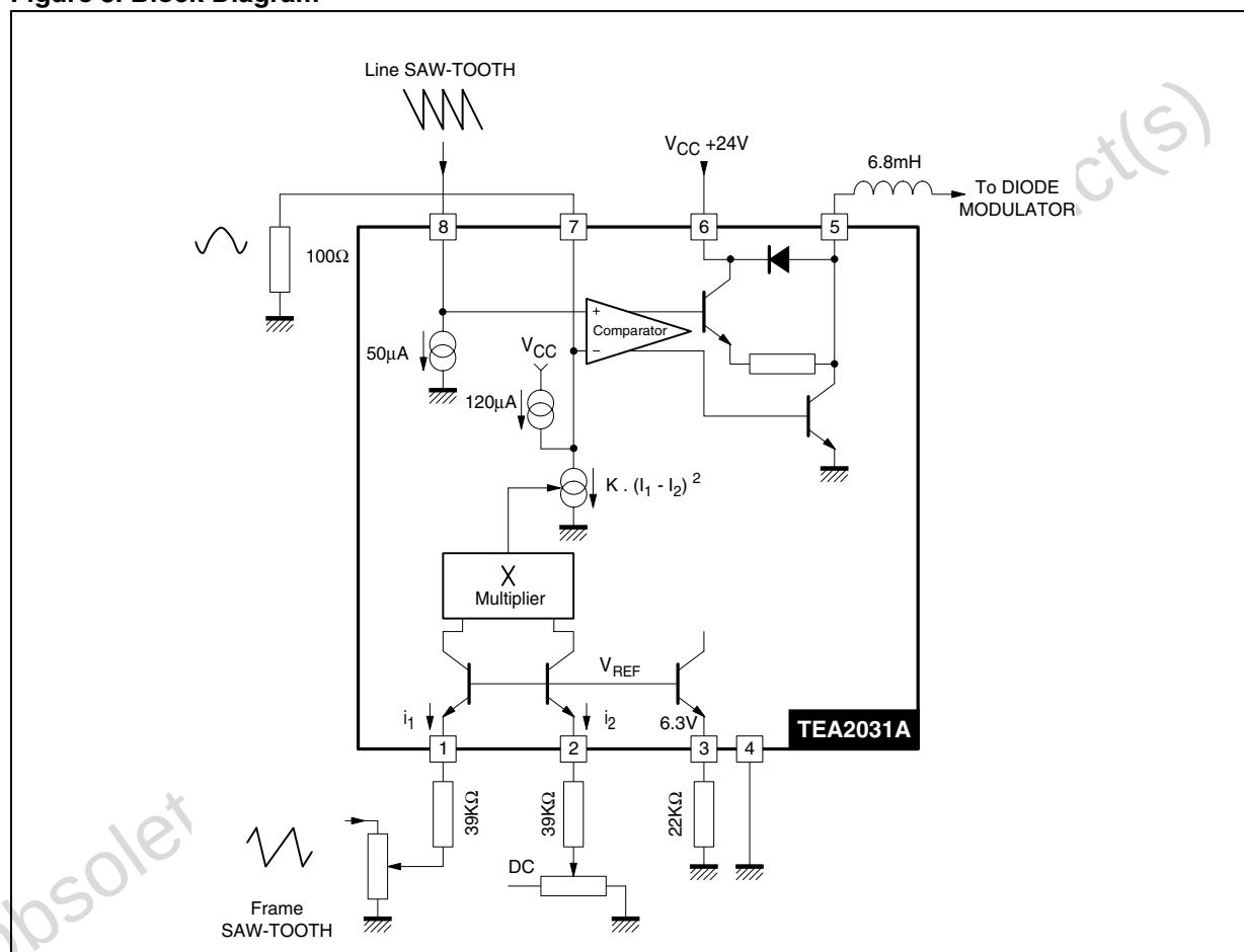
Figure 3. Block Diagram
