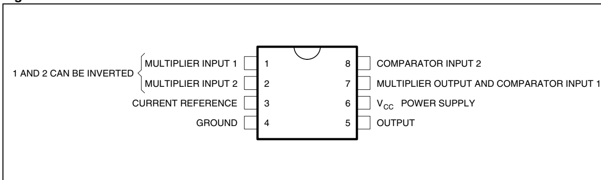
Figure 2. Pin Connections
