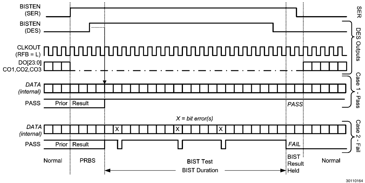
FIGURE 27. BIST Waveforms
