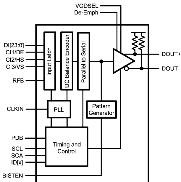
DS92LV2421 – SERIALIZER
