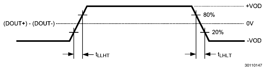
FIGURE 3. Serializer Output Transition Times
