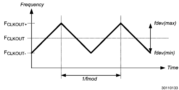
FIGURE 20. SSCG Waveform
