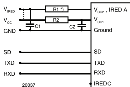
Figure 1. Recommended test circuit.
