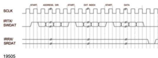
Figure 19. Write Data Waveform with Extended Index
