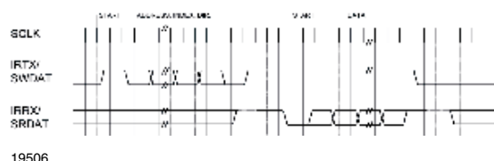
Figure 20. Read Data Waveform
