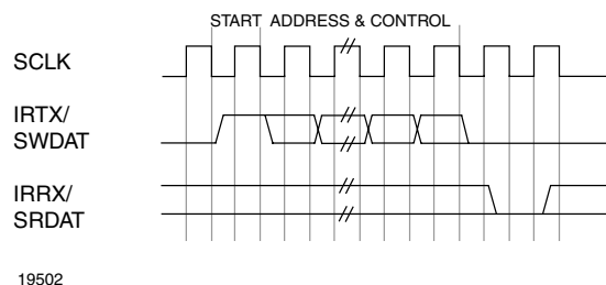
Figure 16. Special Command Waveform
