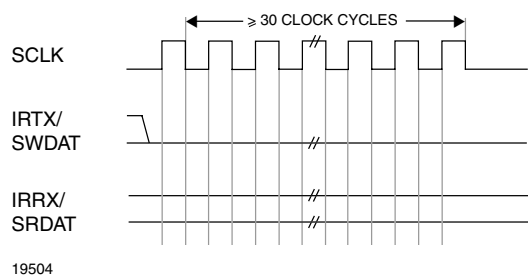
Figure 18. Initial Reset Timing
