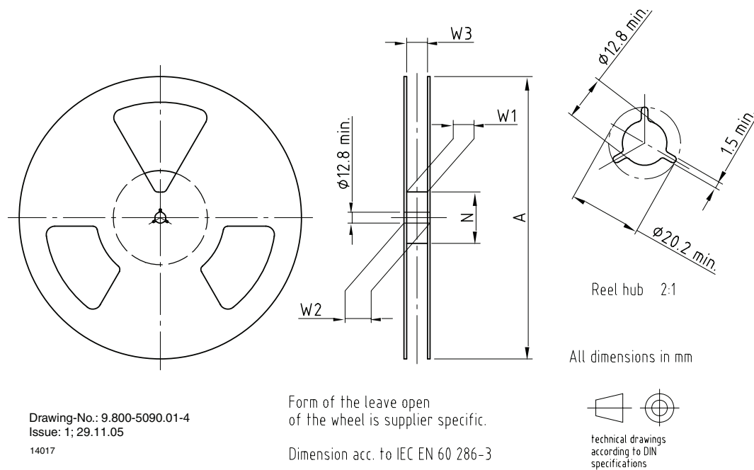
Figure 10. Reel dimensions, dimensions in mm, tolerance \pm 0.2 mm
