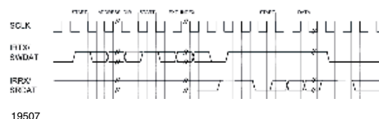
Figure 21. Read Data Waveform with Extended Index
