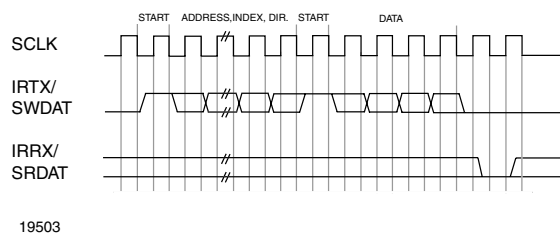
Figure 17. Write Data Waveform
