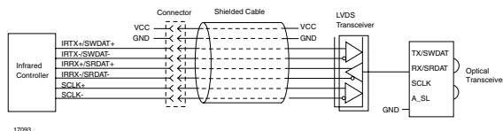
Figure 15. Infrared Dongle with Differential Signaling
