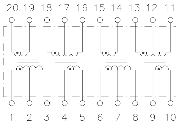
Circuit B
