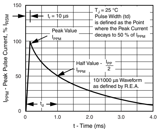
Figure 3. Pulse Waveform
