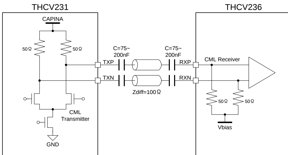
Figure 18. CML Buffer Equivalent Circuit
