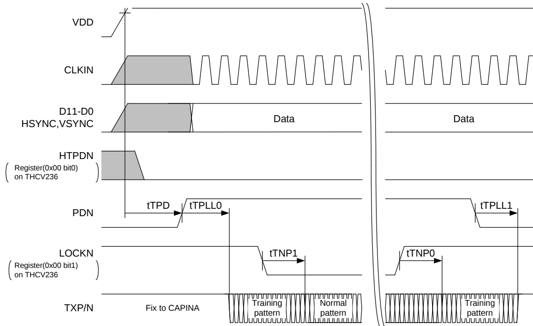
Figure 23. THCV231 Lock/Unlock Sequence
