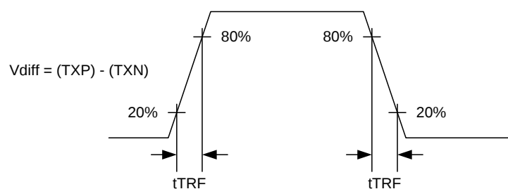
Figure 17. CML Output Switching Characteristics
