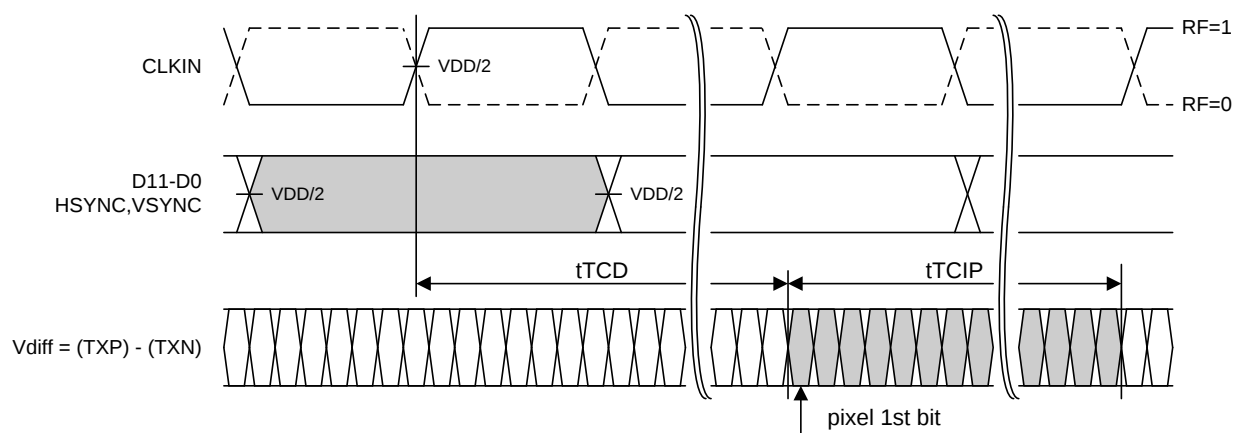
Figure 21. THCV231 Latency
