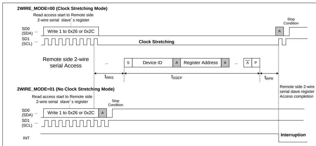
Figure 29. Read access completion time to Remote side 2-wire serial slave register
