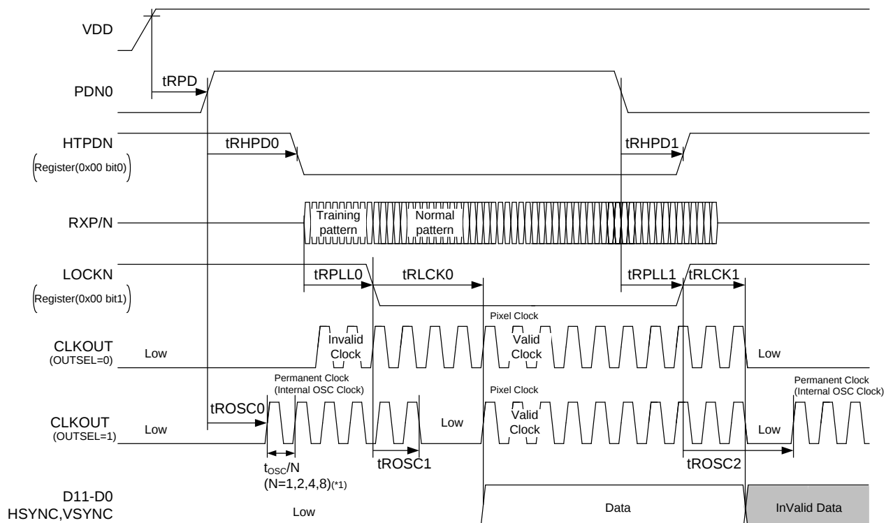
Figure 23. THCV231 Lock/Unlock Sequence
