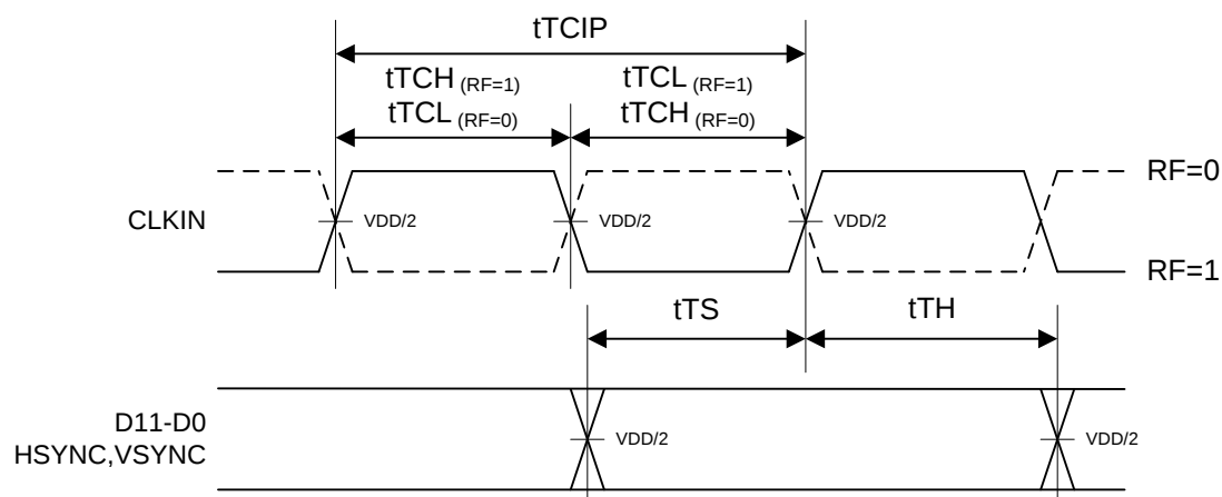
Figure 15. LVC MOS Input Switching Timing Diagrams
