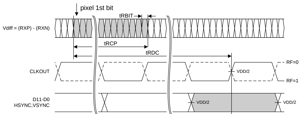
Figure 22. THCV236 Latency
