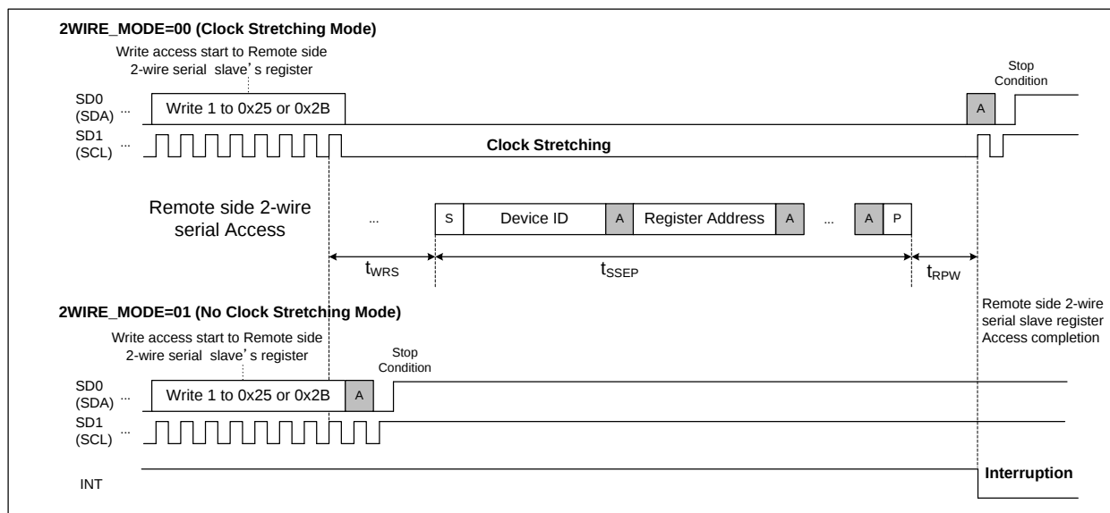
Figure 28. Write access completion time to Remote side 2-wire serial slave register
