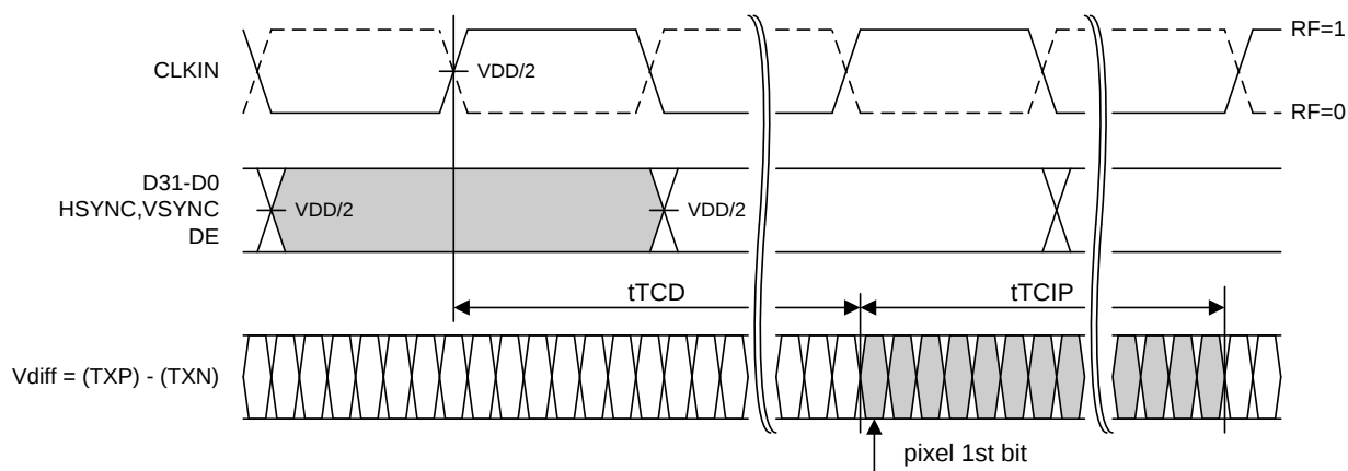
Figure 25. THCV235 Latency
