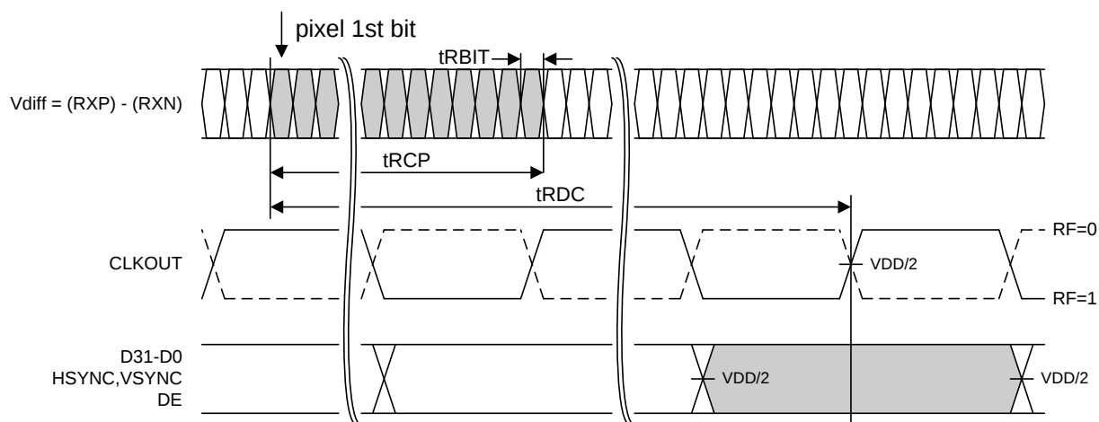
Figure 26. THCV236 Latency
