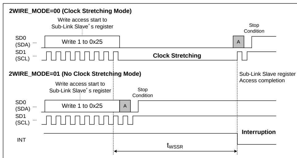
Figure 30. Write access completion time to Sub-Link Slave register
